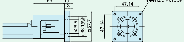
Motor Adaptor Flange F4
