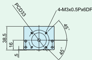
Motor Adaptor Flange F2
