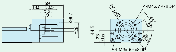
Motor Adaptor Flange F0
