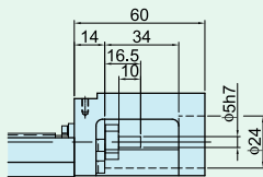
Motor Adaptor Flange F0
