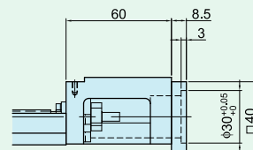
Motor Adaptor Flange F2
